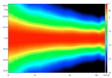
VERTICAL BEAMWIDTH
