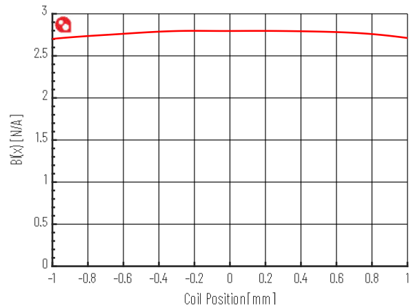
Figure 9 Force Factor B_l vs. Coil Position
