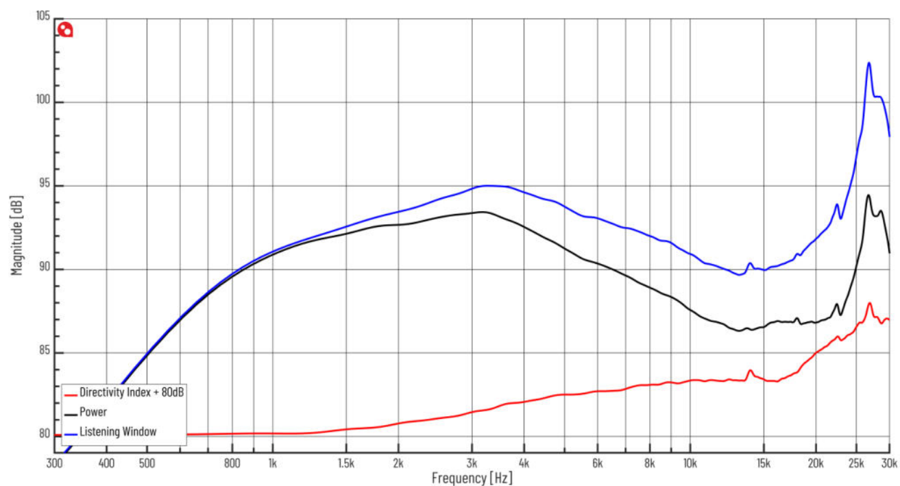
Figure 4 Frequency Response @ 2.83Vrms
