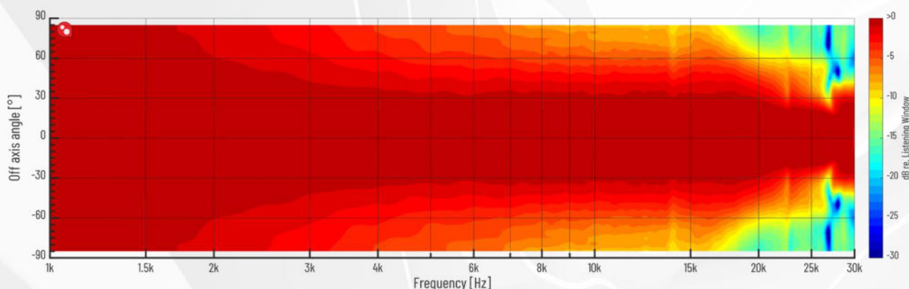
Figure 1 Polar Response normalized to the Listening Window
