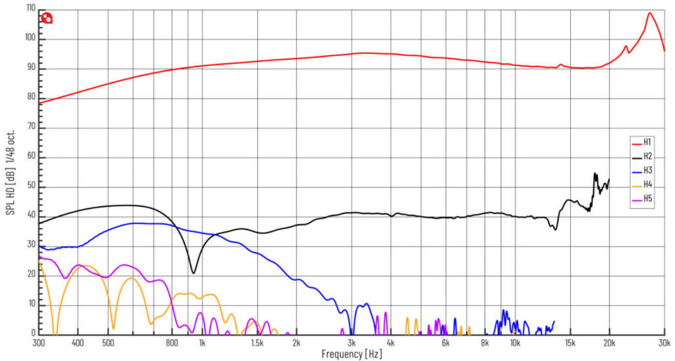
Figure 2 Frequency Response @ 1m, 2.83Vrms
