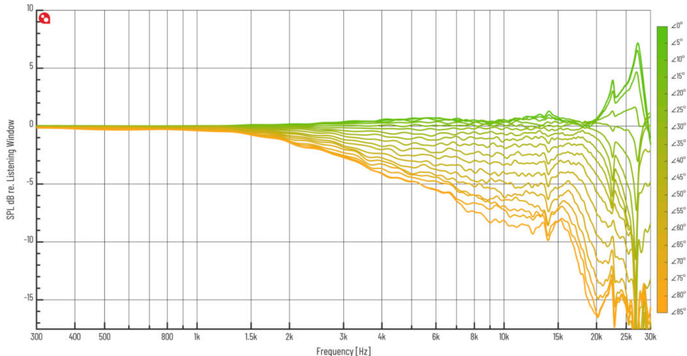
Figure 5 Polar Frequency response relative to the Listening Window
