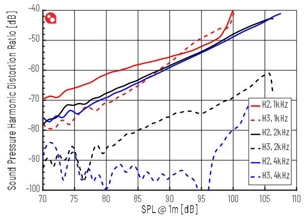
Figure 11 Sound Pressure Harmonic Distortion, C-14Vrms
