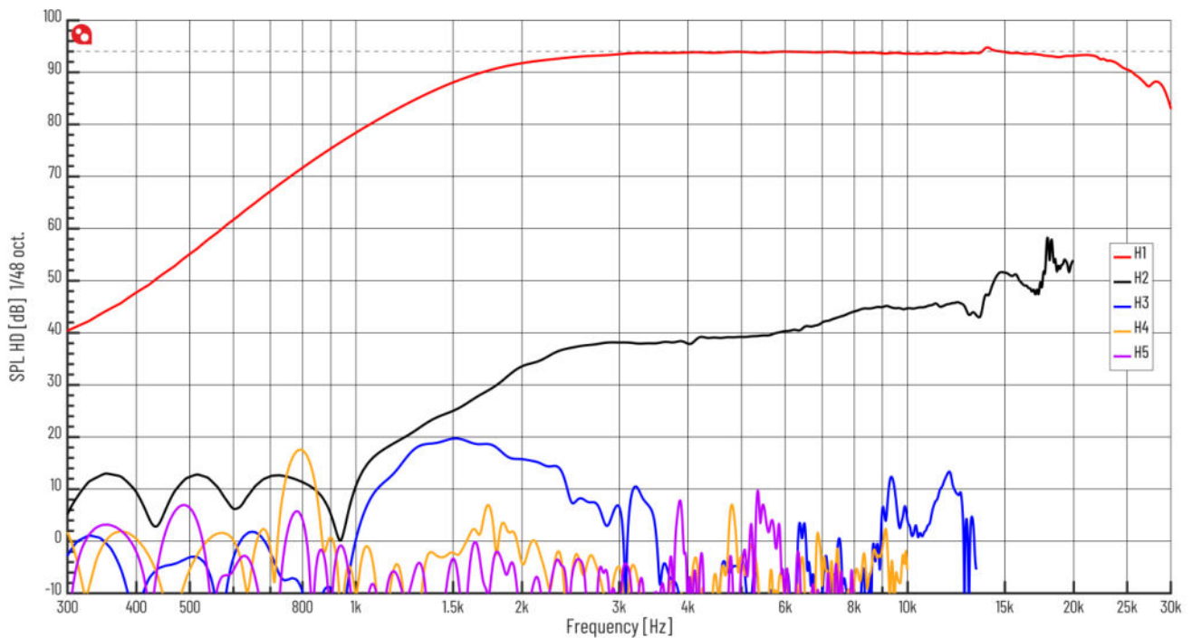
Figure 7 Frequency Response, 94dB, stimulus EQ'd for acoustic 1.5 kHz 4 th -order Linkwitz Riley High-Pass
