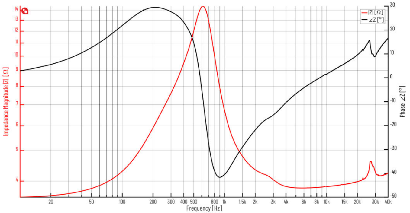
Figure 6 Impedance Response @ 1.41 Vrms, Unsmoothed
