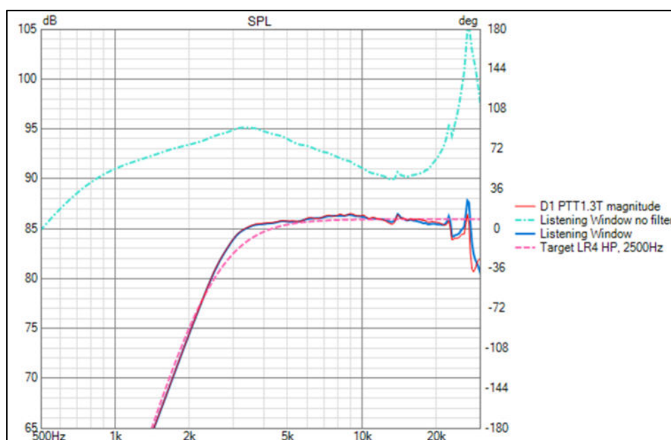
Figure 15 Response Graph from Vituix CAD
