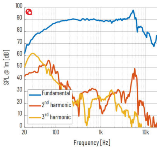
Figure 5 Frequency Response @ 1m, 90dB
