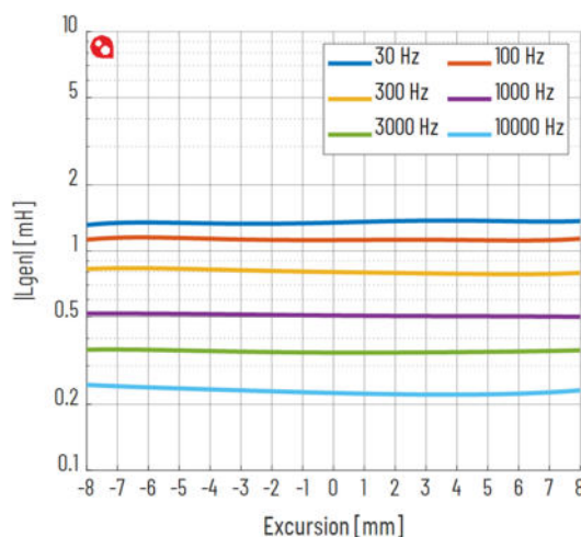
Figure 3 Inductance vs Voice Coil Position
