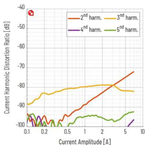
Figure 7 Current Harmonic Distortion @ 1kHz, 0-28.3Vrms
