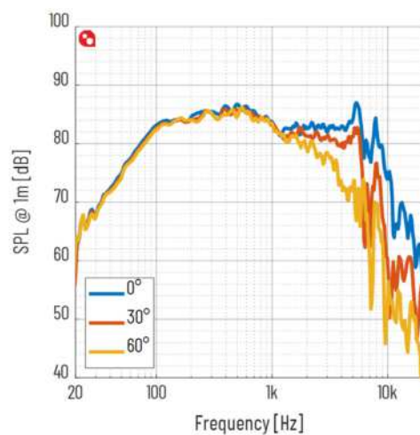
Figure 4 Axial Frequency Response @ 1m, 2.83Vrms
