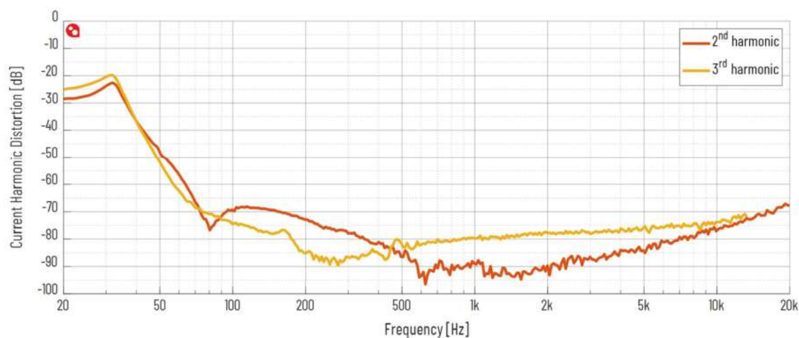
Figure 6 Current Harmonic Distortion @ 2.83Vrms
