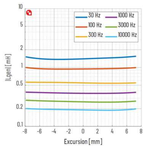
Figure 3 Inductance vs Voice Coil Position
