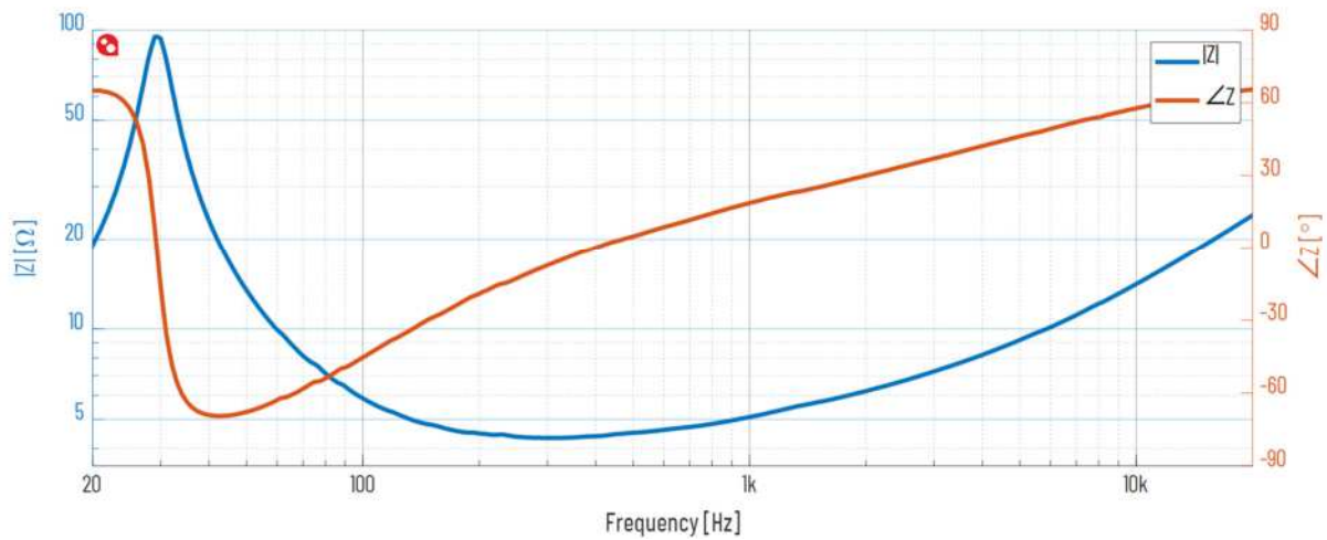
Figure 1 Impedance Response @ 2.83V
