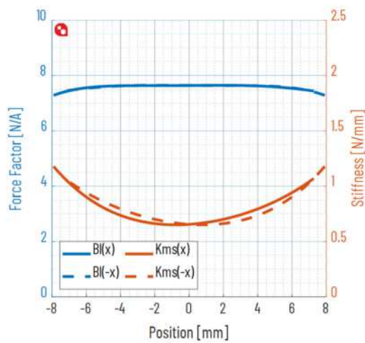
Figure 2 Force Factor and Stiffness vs Voice Coil Position
