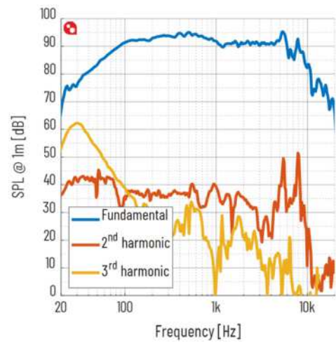
Figure 5 Frequency Response @ 1m, 94dB
