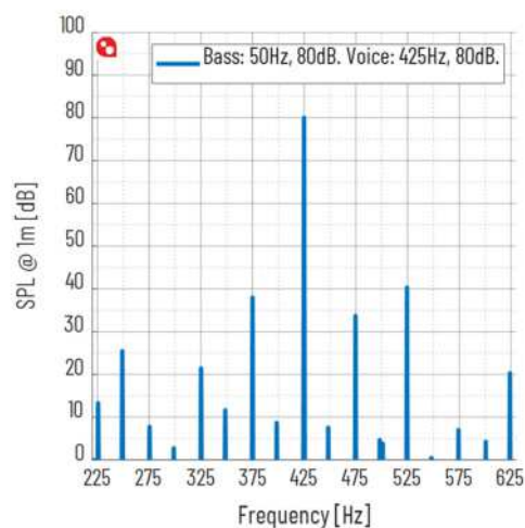
Figure 9 Intermodulation Distortion @ 50Hz 80dB, 425Hz 80dB
