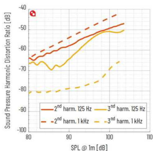
Figure 8 Sound Pressure Harmonic Distortion @ 1m, 0-28.3Vrms
