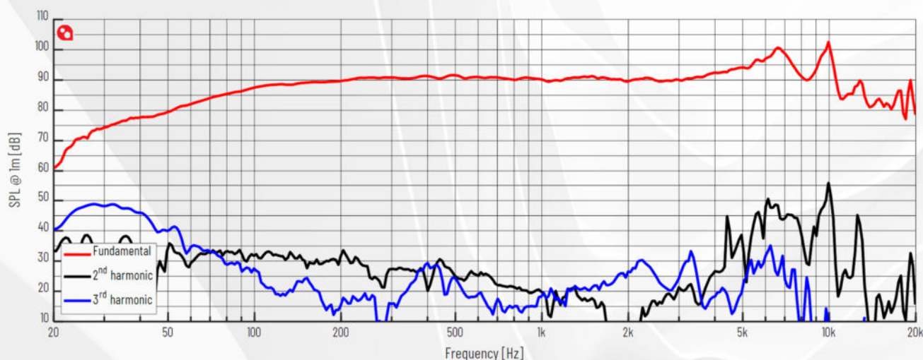
Figure 1 Frequency Response 2.83Vrms @1m
